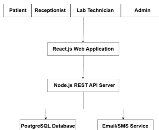
Overall Architecture of the Proposed Laboratory Information System
